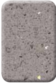
Lunar Ice
